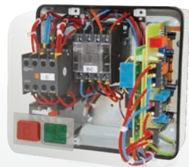
3DC3ENS S10 DC Injection Brake (Driver Card)
