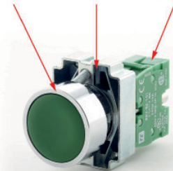
Start Button + Coupler + 1 x NO Contact PB013C + PB093C + PB039C
